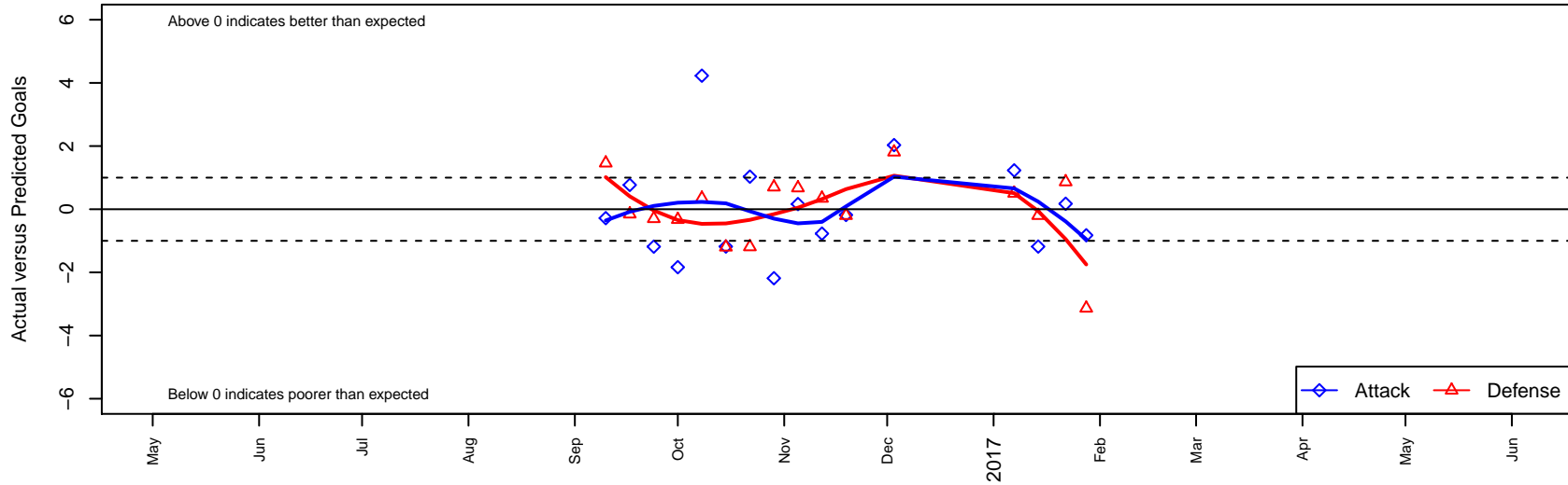
Highline SA B03 Dots are actual minus expected GF (blue circles) and GA (red triangles). Blue line is smoothed change in attack strength. Red is smoothed change in defense strength.
